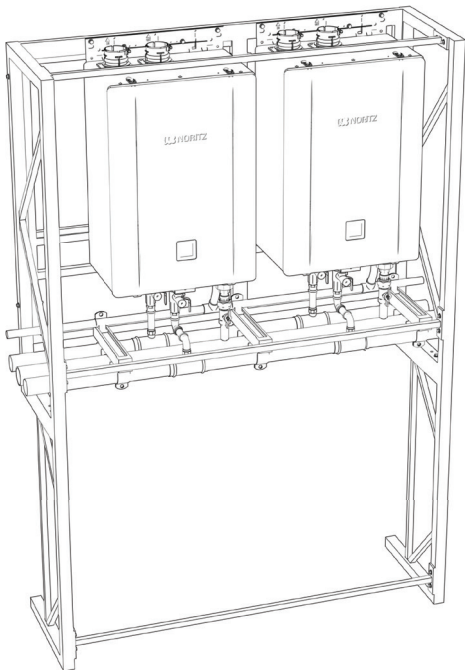
Illustrated: CR61-WH-2 (shown with optional floor support)
