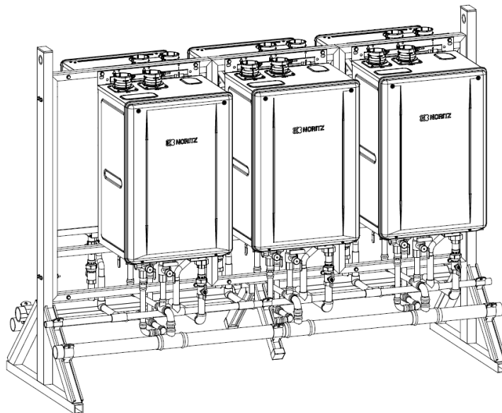
Illustrated: CR60-FS-6
